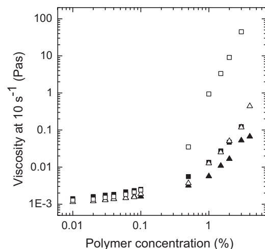
Fig. 1. Viscosity at a shear rate of 10 \text{s}^{-1} as a function of pectin concentration at pH 5 (triangles) and pH 3 (squares) for pectin with similar degree of methylation but with random (solid symbols) and blocky (open symbols) charge distribution.
