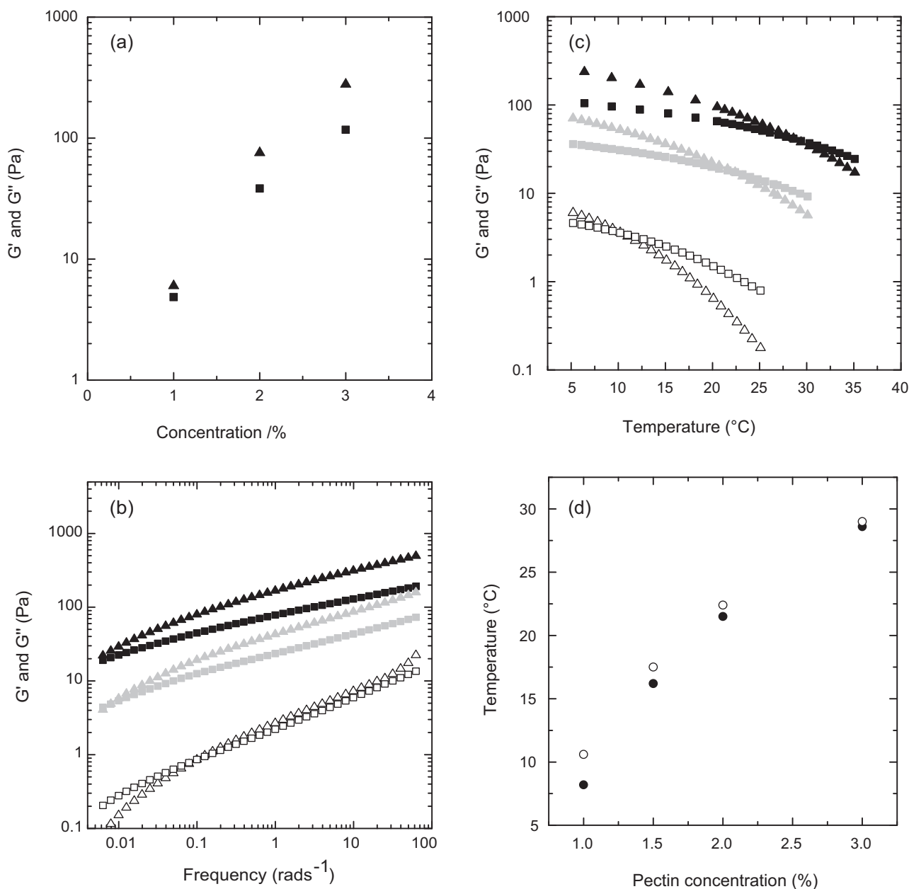
Fig. 2. Oscillatory rheology on blocky pectin gels, where G' (triangles) and G'' (squares) of pectin samples at pH 3 and as a function of (a) pectin concentration at T = 5^\circ\text{C} ; (b) frequency sweep where black symbols represent 3% pectin, gray 2% pectin and open 1% pectin at T = 5^\circ\text{C} ; (c) temperature reduction where black symbols represent 3% pectin, gray 2% pectin and open 1% pectin; and (d) temperature at which G' = G'' upon temperature reduction (filled symbols) and temperature increase (open symbols) of pectin samples. All tests were performed at T = 5^\circ\text{C} , f = 6.28 \text{ rad/s} , \text{pH} = 3 and strain = 0.5%, unless otherwise indicated.
